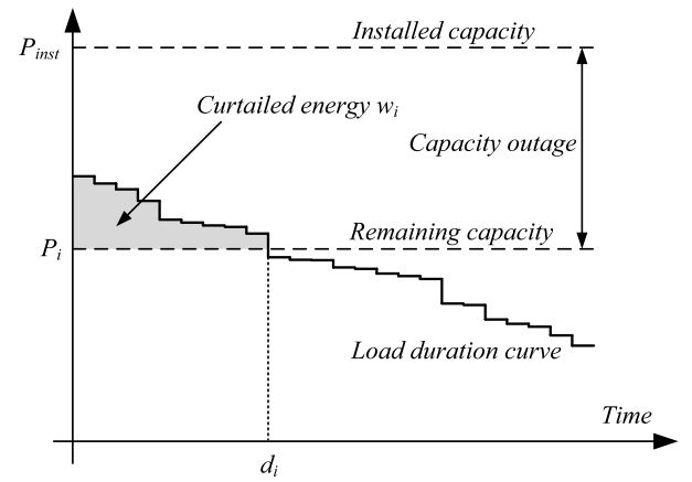
Fig. 1. Load duration curve with d_i and w_i .
