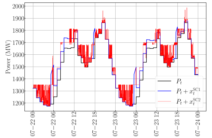
Fig. 11. Total electricity consumption in CS1 and CS2.
